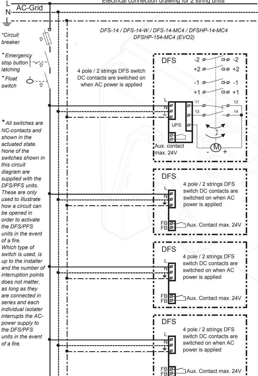
Electrical connection drawing for 2 string units
