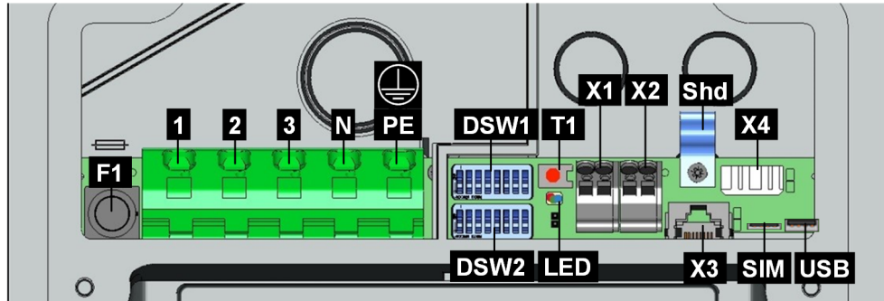
Fig. 7-16: Connection overview
