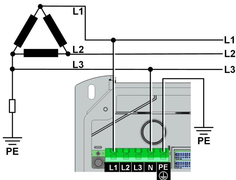
Fig. 7-19: Connection to a three-wire IT system with 230 V
