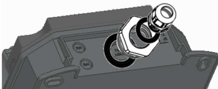
Fig. 7-18: Use of a reducing insert
