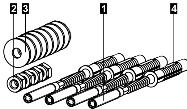
Fig. 3-3: Mounting set for wall installation
