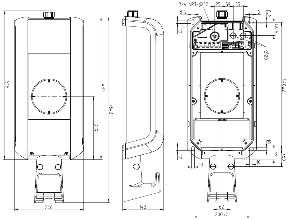
Fig. 12-24: Dimensions in millimeters
